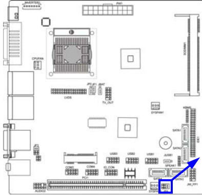
JP4
